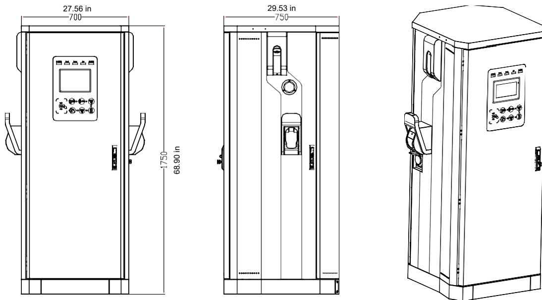
Figure 12: EVSE 3 Views
