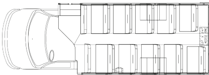
DH500 28 Passenger
